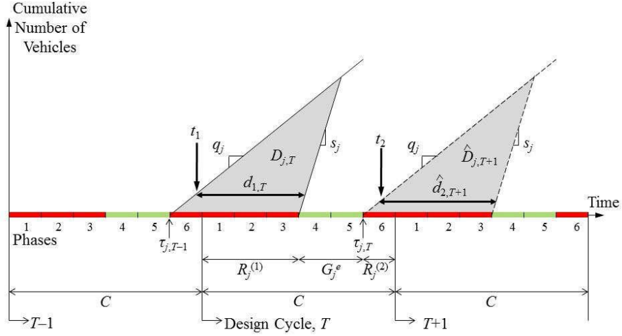
Figure 3.1: Queuing diagram for lane group j for undersaturated conditions, (Source: Christofa et al. (2013))
