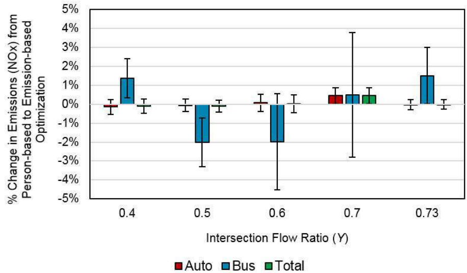
Figure 4.30: Percent change in NOx emissions from person-based to emission (NOx)-based optimization for the intersection of University and San Pablo Avenues (stochastic arrival tests)
