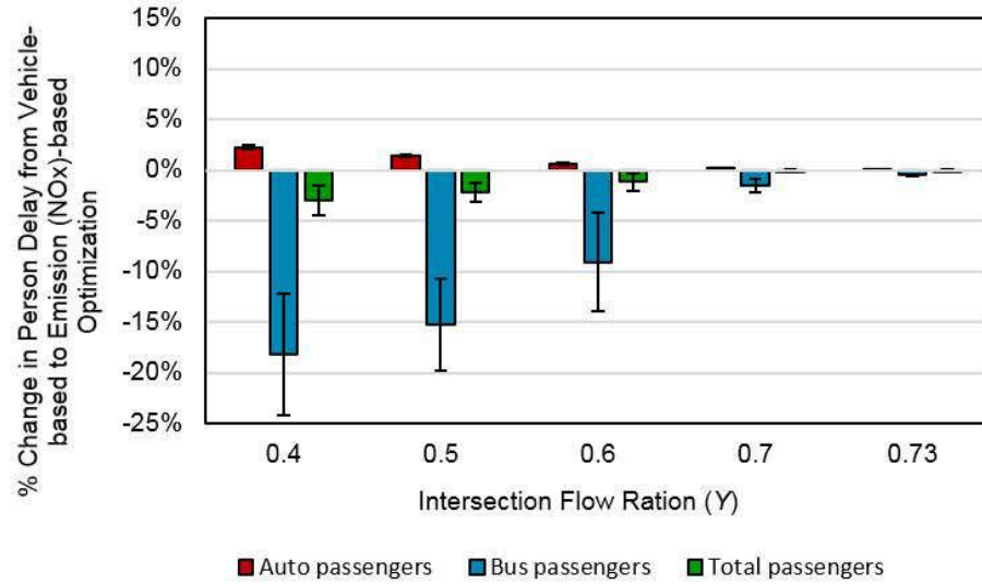
Figure 4.31: Percent change in person delay from vehicle-based to emission (NOx)-based optimization for the intersection of University and San Pablo Avenues (deterministic arrival tests)
