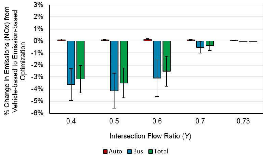
Figure 4.27: Percent change in NOx emissions from vehicle-based to emission (NOx)-based optimization for the intersection of University and San Pablo Avenues (deterministic arrival tests)
